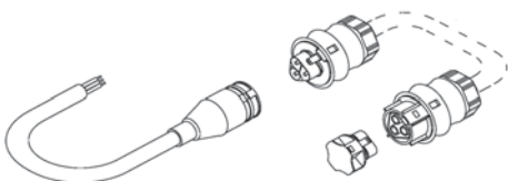
pic.: finishing set HBRA option 3: for direct connection to a power supply line
